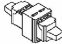
Duplex LC MM Dimensions: 23.5mm x 17.8mm x 25.7mm (.93"H x .70"W x 1.01"D) Shipping Weight: 12g (.43 oz.)
