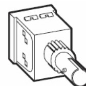
ST SM/MM Dimensions: 23.5mm x 17.8mm x 29.1mm (.93"H x .70"W x 1.15"D) Shipping Weight: 10.7g (.38 oz.)
