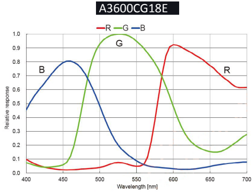
Quantum Efficiency Curve for Mono and Color
